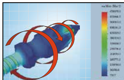
PROJAHN TORSION-Bit
