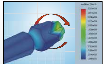
Standard-Bit
