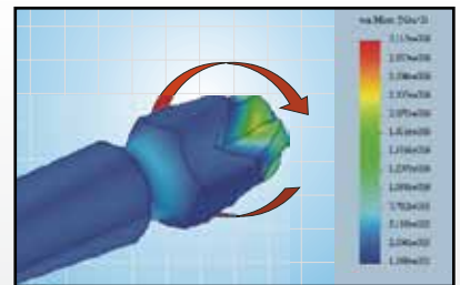
Standard-Bit
